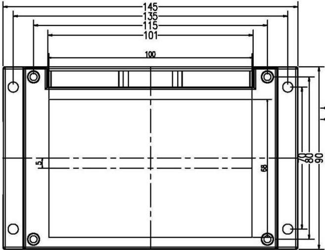
Figure 5: Enclosure drawing. Measurements in mm
